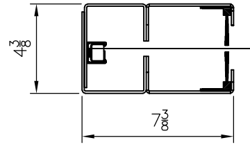
TRACK DETAIL 4:1
