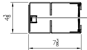
TRACK DETAIL 4:1
